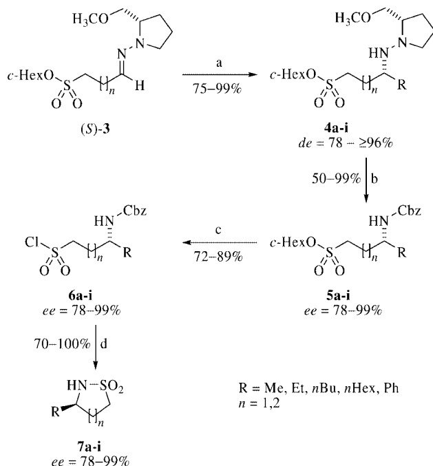
Scheme 2. Asymmetric synthesis of \gamma - and \delta -sultams 7 . Reagents and conditions: a) RM/ \text{CeCl}_3 , THF, -100^{\circ}\text{C} to -78^{\circ}\text{C} , 3 h; b) 1. \text{BH}_3\cdot\text{THF} , THF, reflux, 4 h; 2. \text{CbzCl} , \text{K}_2\text{CO}_3 , \text{CH}_2\text{Cl}_2 , reflux, 18 h; c) 1. \text{EtOH}/\text{H}_2\text{O} , reflux, 18 h; 2. \text{NaOAc} , \text{CH}_2\text{Cl}_2 , room temp., 1 h; 3. \text{COCl}_2 in toluene, \text{CH}_2\text{Cl}_2/\text{DMF} , room temp., 2 h; d) 1. \text{HBr}/\text{AcOH} , \text{CH}_2\text{Cl}_2 , room temp., 3 h; 2. \text{NEt}_3 , 0^{\circ}\text{C} , 2 h.
